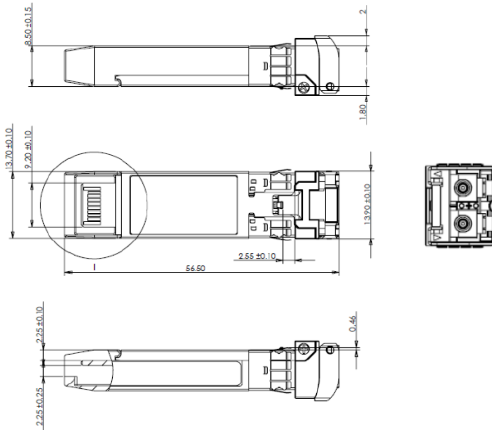
Figure 4. Mechanical Outline
